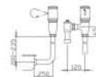
AUTOMATIC TOILET FLUSHER HL-5601
